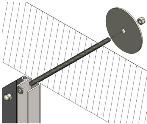
Aerated autoclaved concrete (maximum wall thickness: 300 mm)
