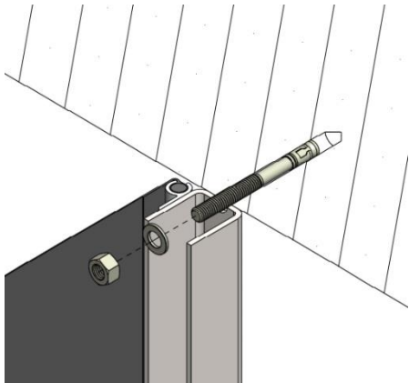
Concrete (heavy duty)
